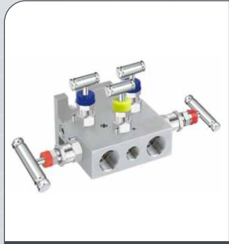
5 Valve Manifold Pipe To Flange (Model No - 5VM-TT-FF) Tee Type
